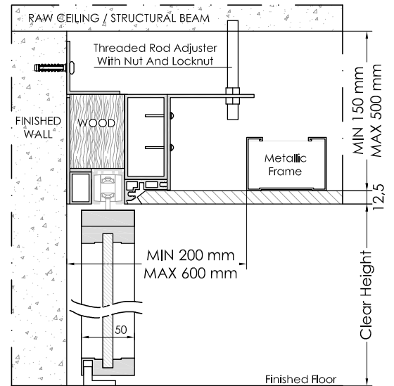
VERTICAL SECTION
